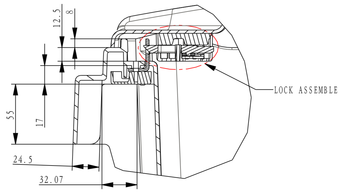
DETAIL B SCALE 0.500
