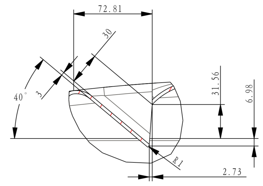
DETAIL A SCALE 0.500
